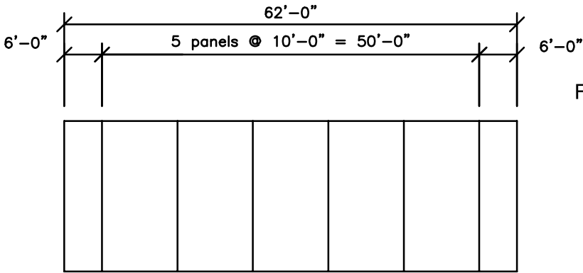
Flat Panel
