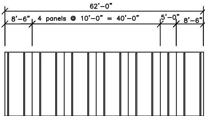
Double Tee Wall Panel
