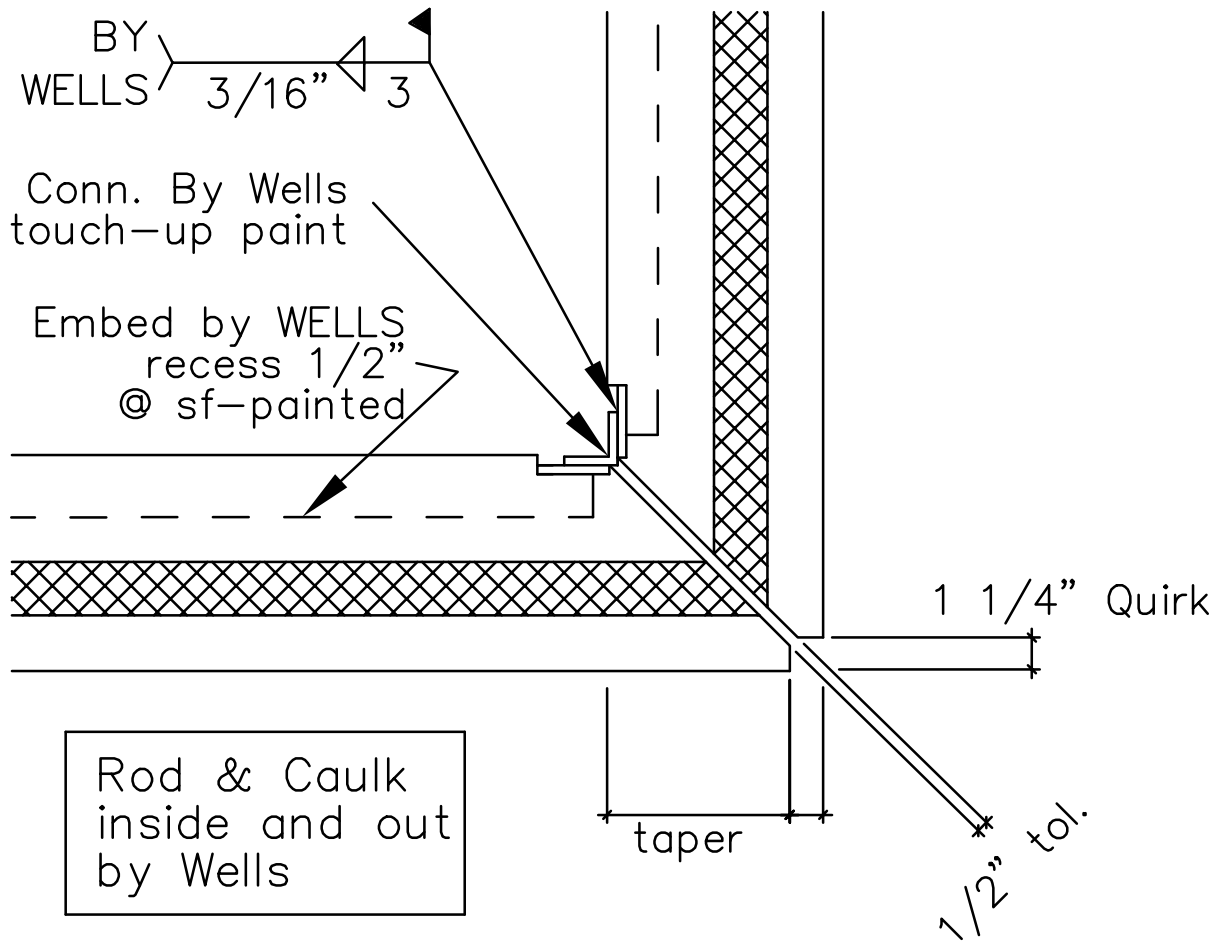
① Detail
