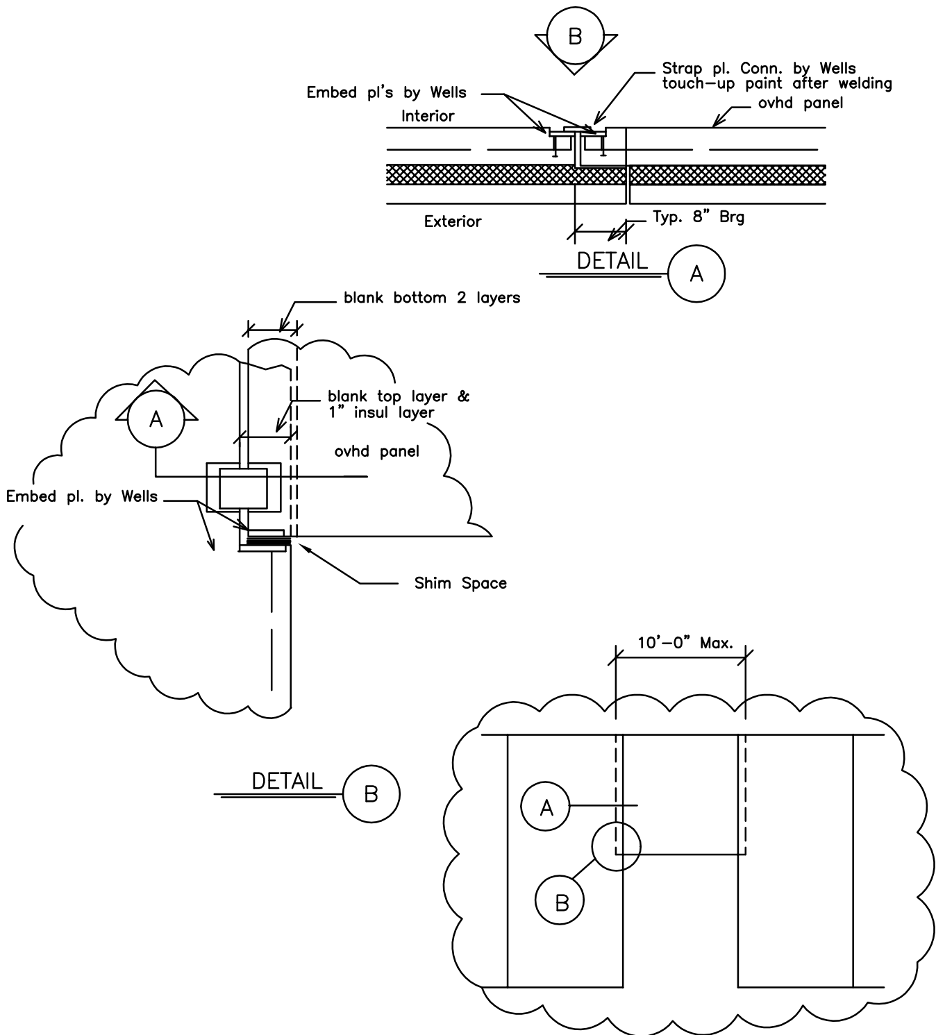
OVHD PANEL BRG ON ADJACENT FULL LGTH PANEL (flat panels only)
